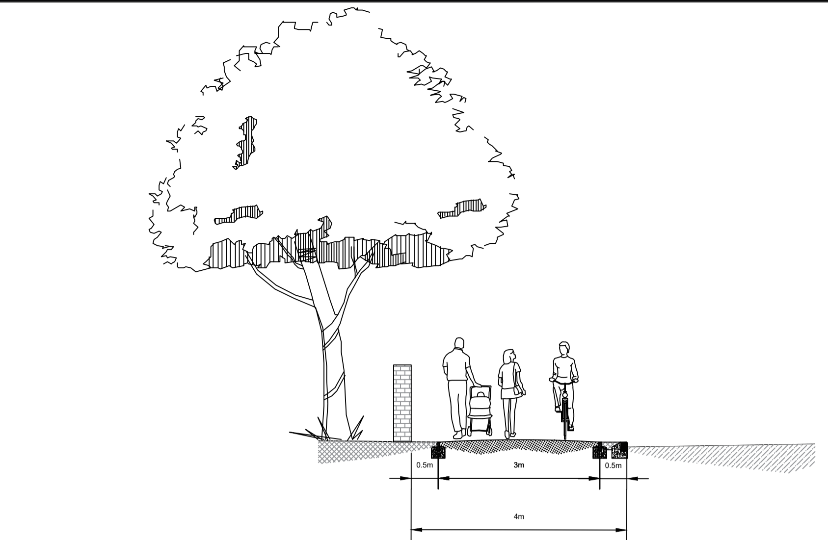
EXAMPLE OF TYPICAL SECTION THROUGH A 3m REDWAY
