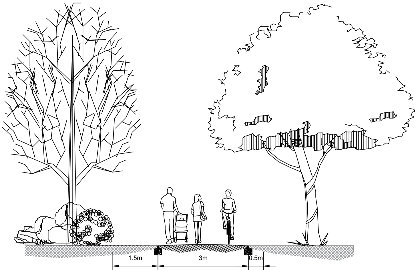
EXAMPLE OF TYPICAL SECTION THROUGH A 3m SHARED REDWAY
