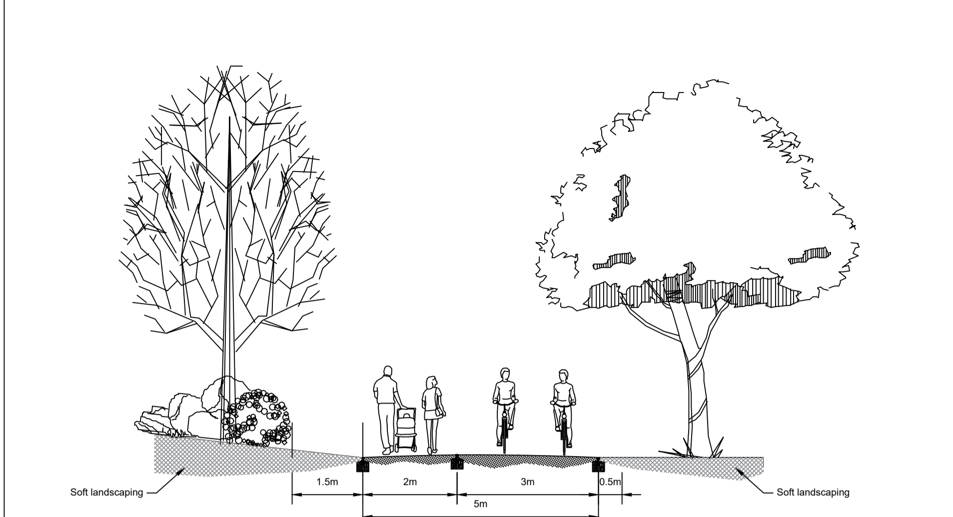
EXAMPLE OF TYPICAL SECTION THROUGH A 5m SEGREGATED REDWAY
